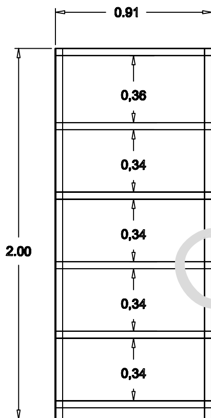
Vista Frontal
