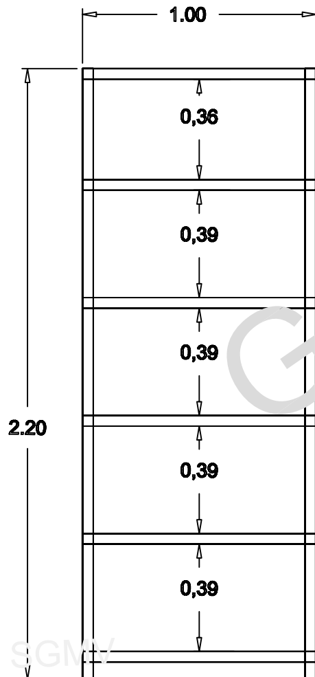
Vista Frontal
