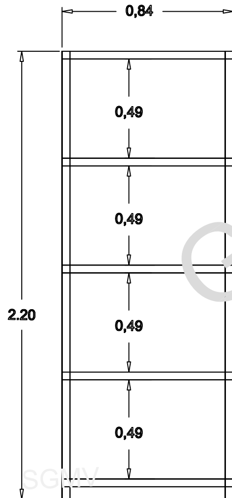
Vista Frontal
