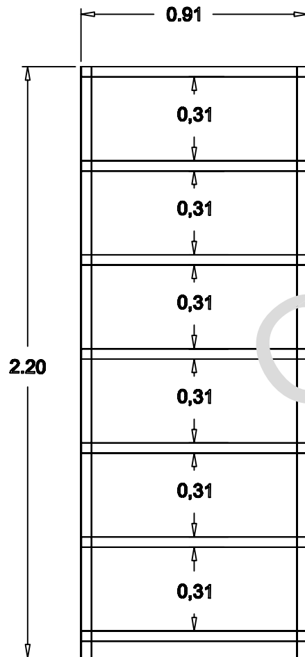
Vista Frontal
