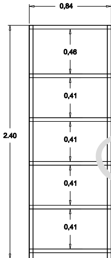
Vista Frontal
