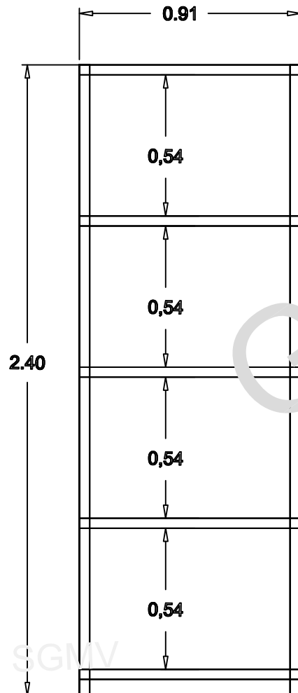
Vista Frontal
