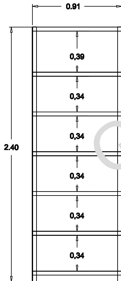
Vista Frontal
