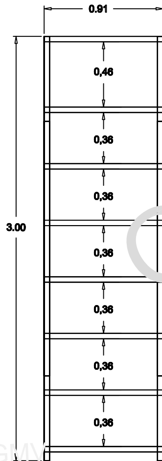
Vista Frontal
