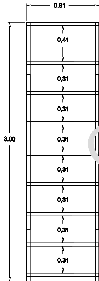
Vista Frontal
