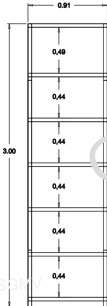
Vista Frontal
